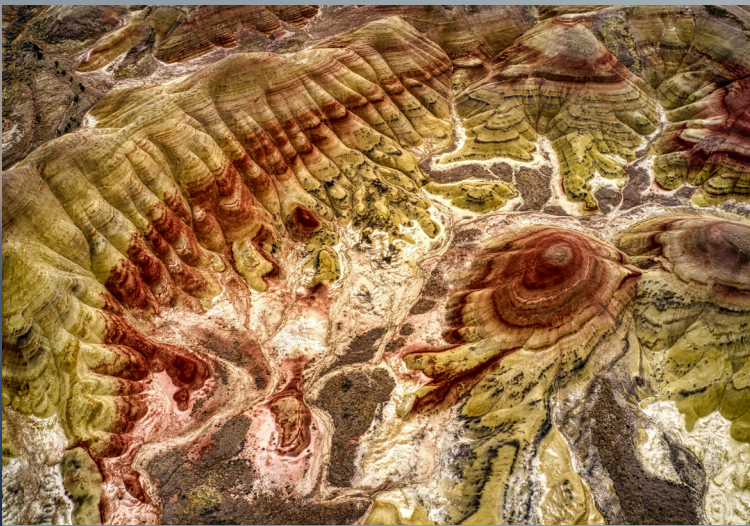
Geodynamic Processes
